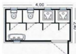
FG12Z40S1 Mt 4,00x2,40x2,45
