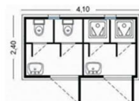
FG12H40S1 Mt. 4,10x2,40x2,45
