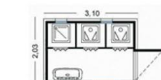
FG12B30S2 Mt. 3,10x2,03x2,45
