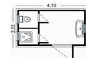
FG12B40S2 Mt. 4,10x2,03x2,45
