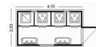
FG12B40S4 Mt. 4,10x2,03x2,45
