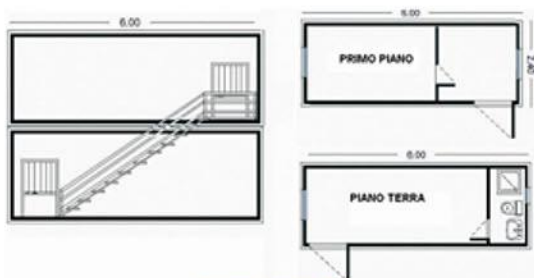
FG12C60S1 Mt. 6,00x2,40x5,70
