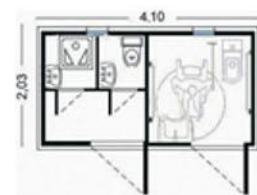
FG12B40S5 Mt. 4,10x2,03x2,85 (disabili)
